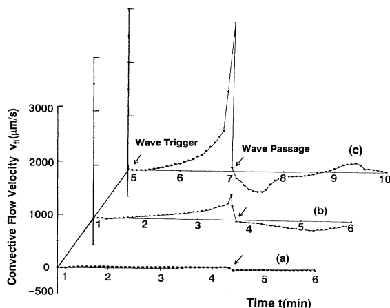
FIG. 3. Temporal traces of hydrodynamic motion velocity ( v_n ) induced by chemical-wave propagation. (a) Ordinary wave triggered at t_{tr}=1 min after mixing; (b) and (c) big waves triggered at t_{tr}=1 and 5 min (10 s immersion), respectively. The velocity v_n associated with the big wave is almost 30 times faster than that of the ordinary wave.
