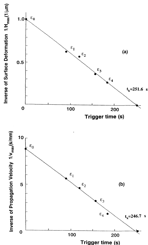
FIG. 6. Inverse of maximum deformation H_{max}^{-1} (a), and of maximum propagation velocity v_{max}^{-1} (b) of the big wave as a function of trigger time t_{tr} . Here, \epsilon_1, \epsilon_2, \epsilon_3, and \epsilon_4 show the measured points. the straight line is determined by linear regression. The values \epsilon_0 and t_k are obtained by extrapolation.
