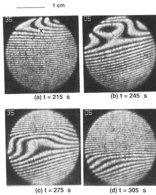
FIG. 4. Distortion of fringe pattern in a Mach-Zehnder interferometer caused by the big wave propagation from the top to the bottom; t_{tr} = 157 s.
