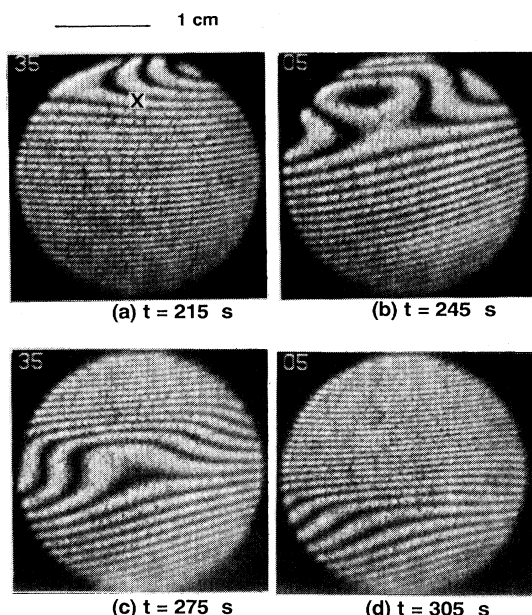
FIG. 4. Distortion of fringe pattern in a Mach-Zehnder interferometer caused by the big wave propagation from the top to the bottom; t_{tr}=157 s.
